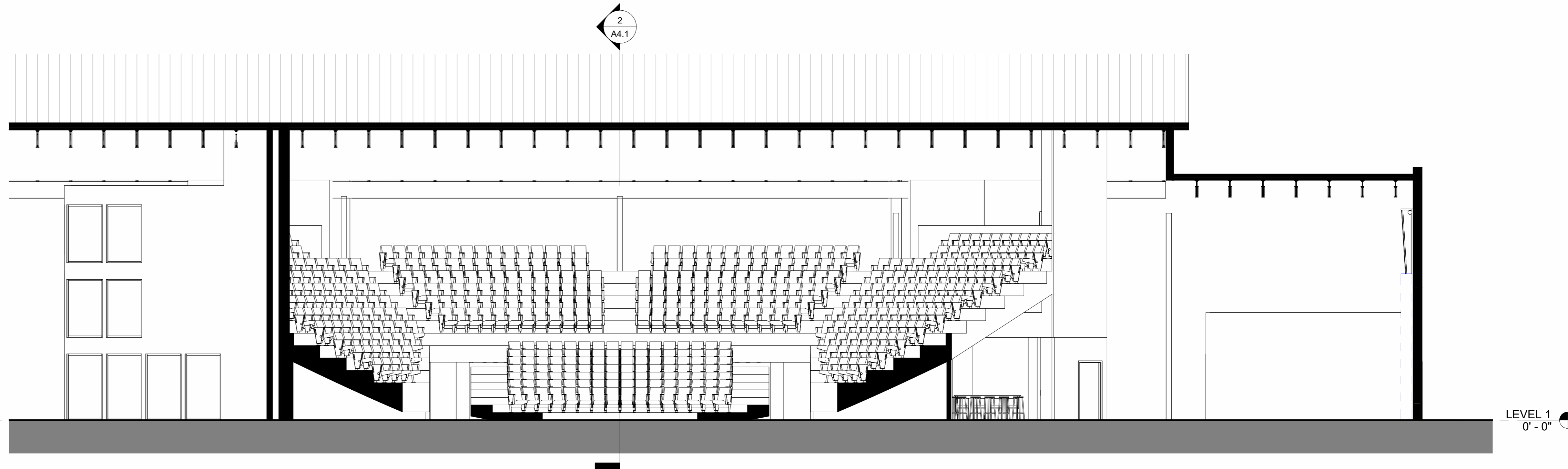
3 SECTION N/S 1/8" = 1'-0" @ FULL SIZE
