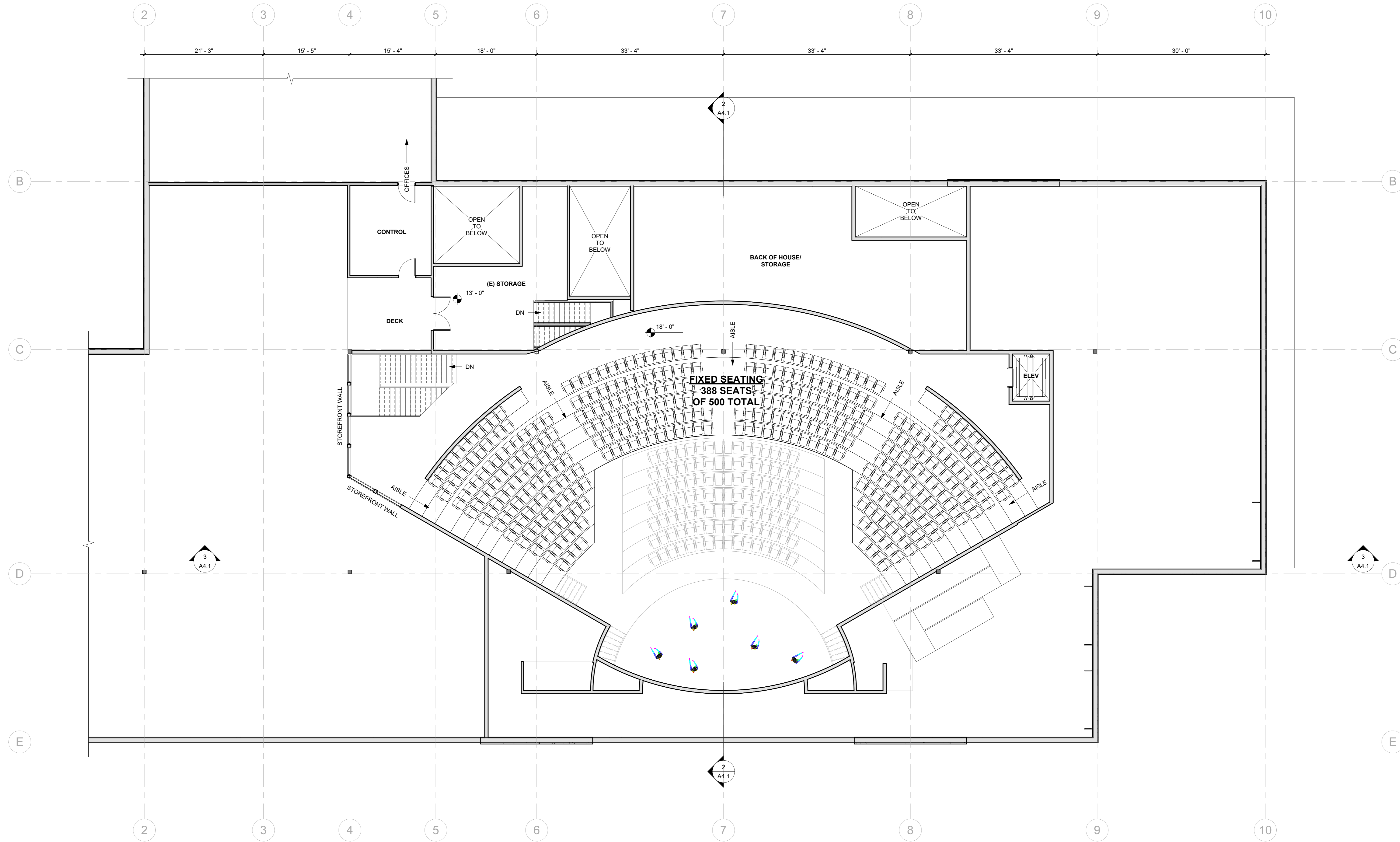
1 BALCONY 1/8" = 1'-0" @ FULL SIZE 0' 2' 4' 8'
