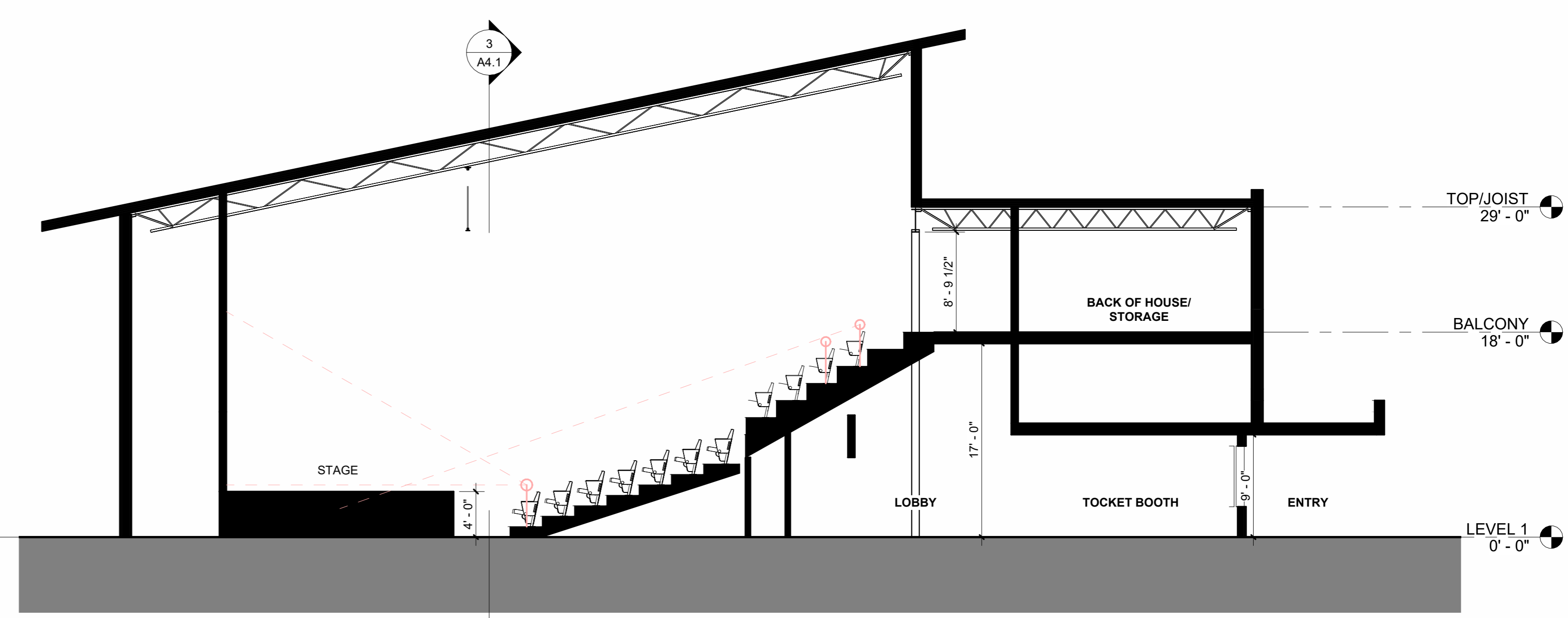
2 SECTION E/W 1/8" = 1'-0" @ FULL SIZE
