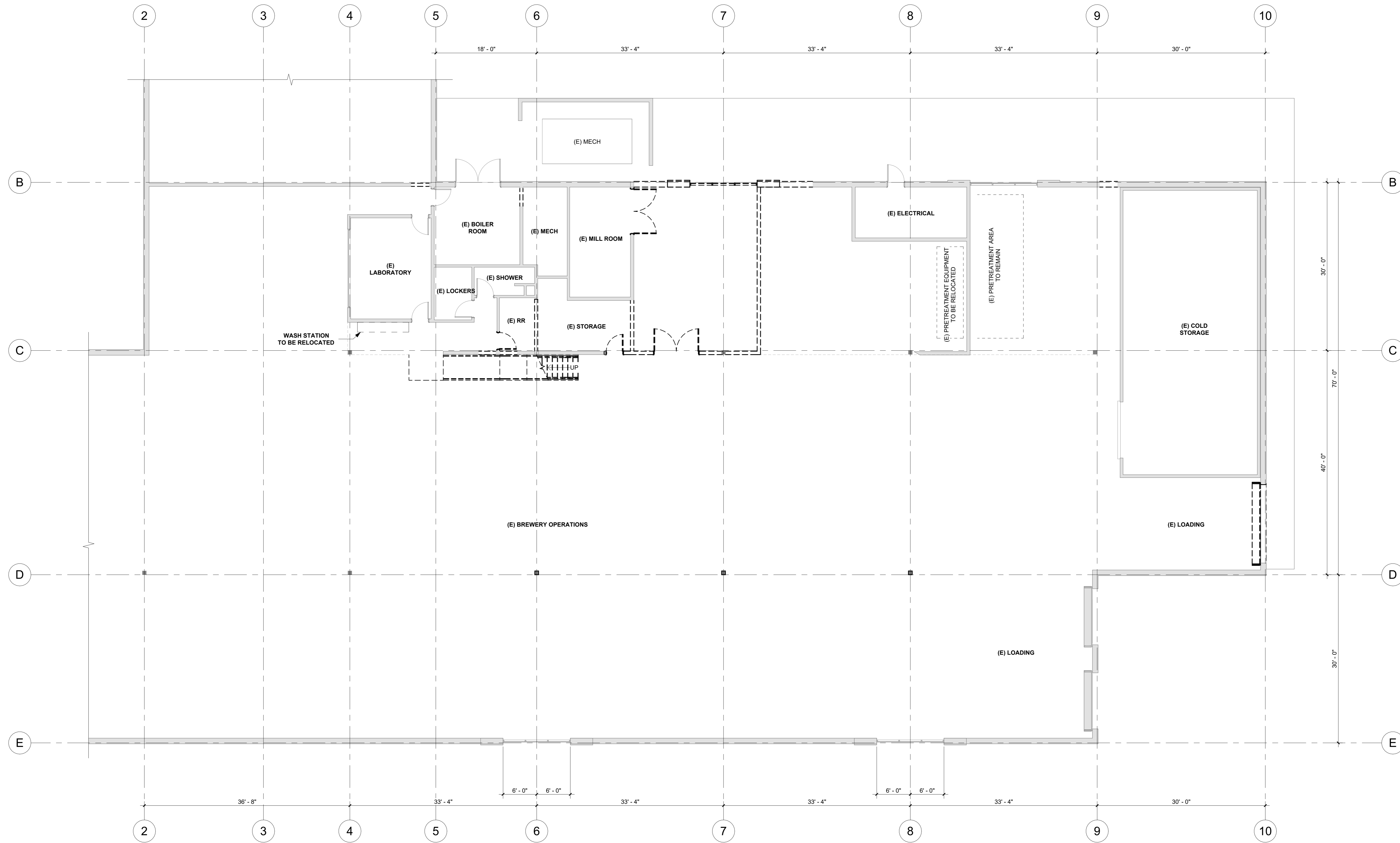
1 DEMOLITION PLAN - LEVEL 1 1/8" = 1'-0" @ FULL SIZE 0' 2' 4' 8'
